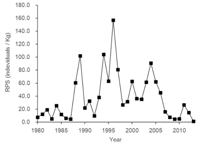
Fig. 6 Recruit per spawning (RPS) of marbled sole in Tokyo Bay, Japan, between 1980 and 2013..
